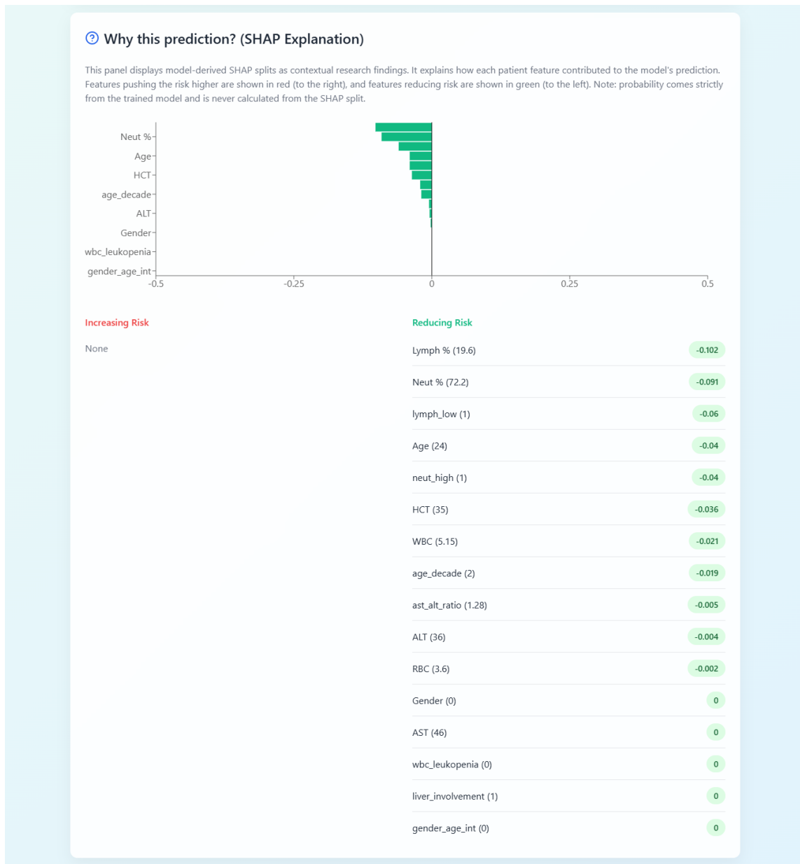
Figure 4.7: Patient-level SHAP explanation showing individual feature contributions to the model output for a selected assessment.
